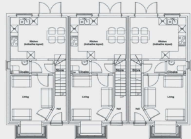
PLOT 3 PLOT 4 PLOT 5 GROUND FLOOR PLAN Scale: 1:100
