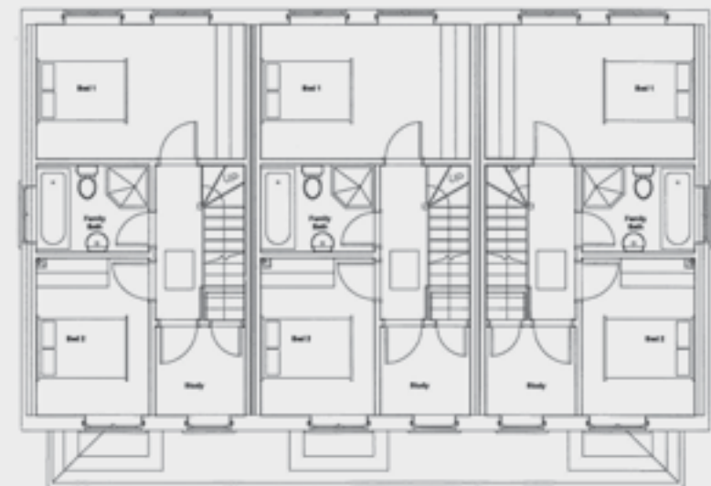
PLOT 3 PLOT 4 PLOT 5 FIRST FLOOR PLAN Scale: 1:100
